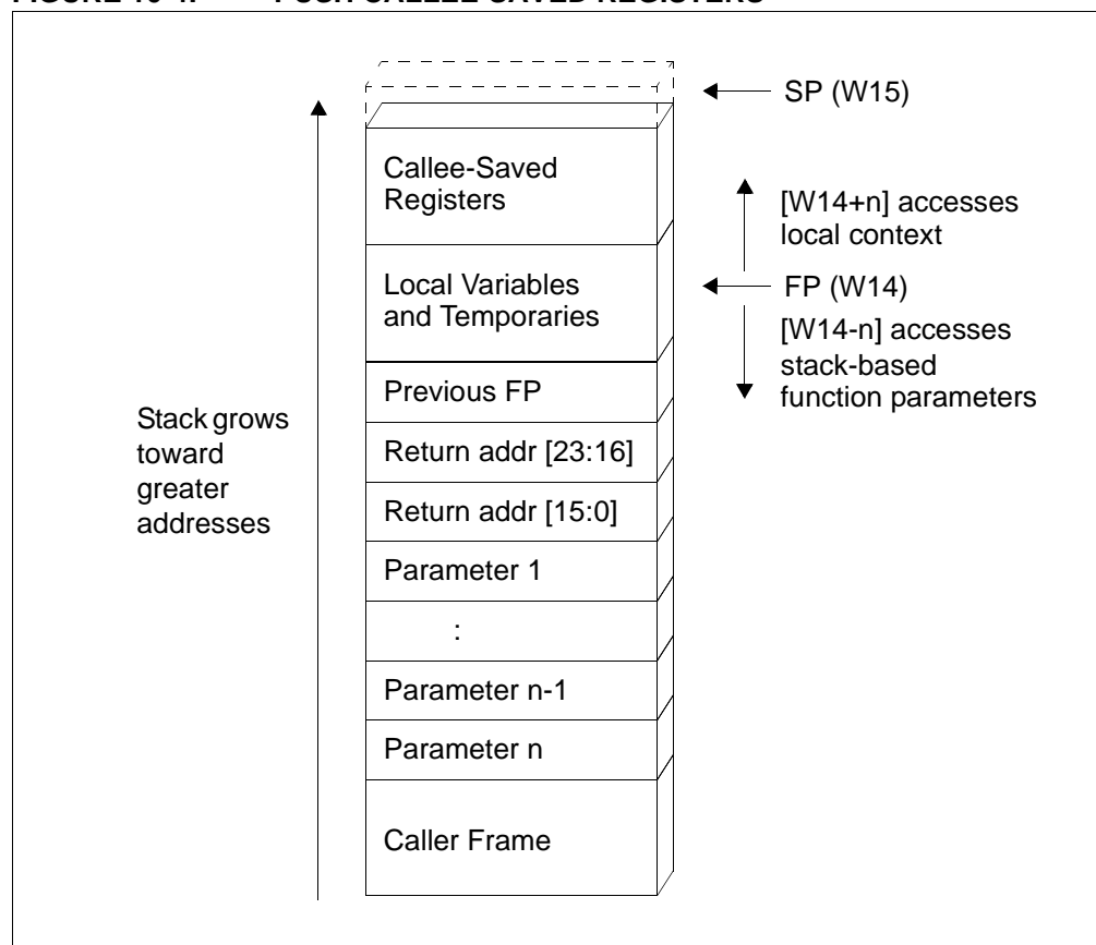
FIGURE 10-4: PUSH CALLEE-AVED REGISTERS
